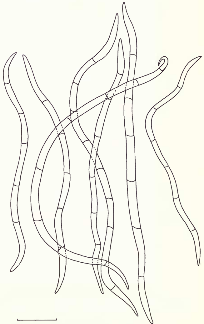
Fig. 30 Ascospore outlines of Celothelium aciculiferum (Nyl.) Vainio (H-NYL 4303-isotype); scale = 10 µm.
